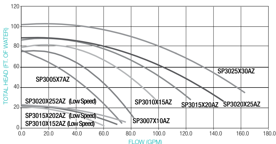
SUPER II FLOW VS. TOTAL HEAD
