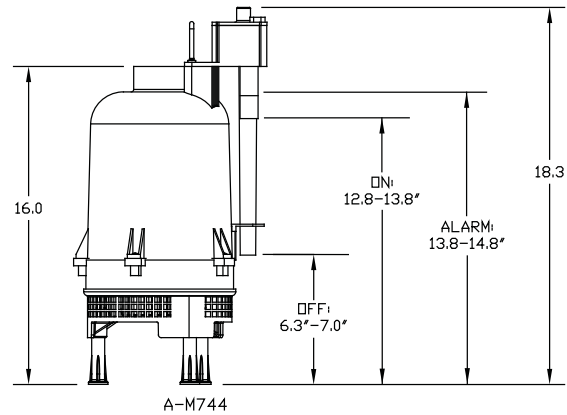
OVERALL DIMENSIONS W/LEG KIT
